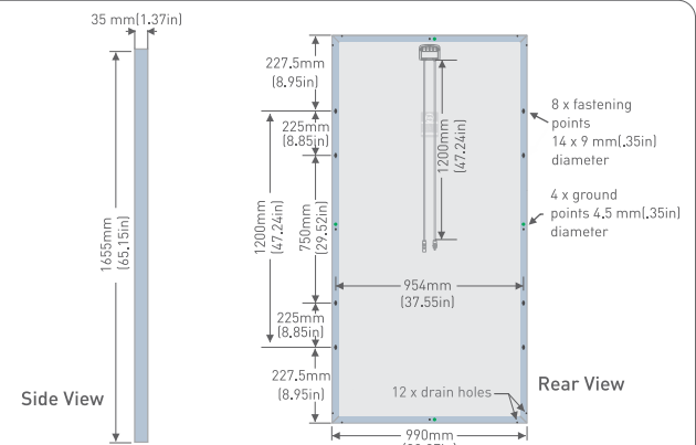
Module Dimension Drawing
