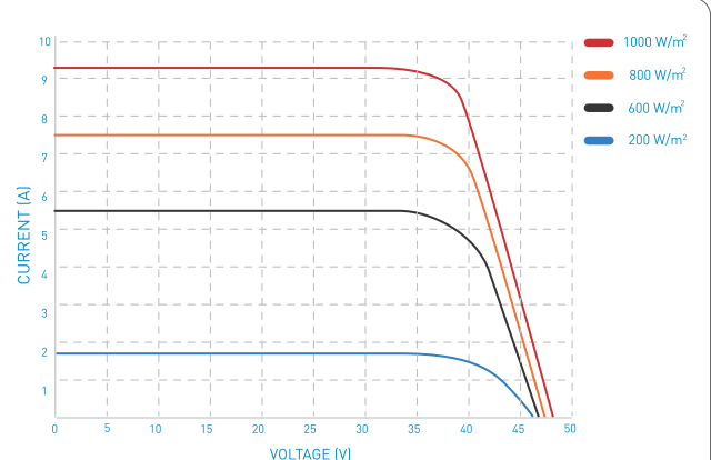
Typical IV Curves
