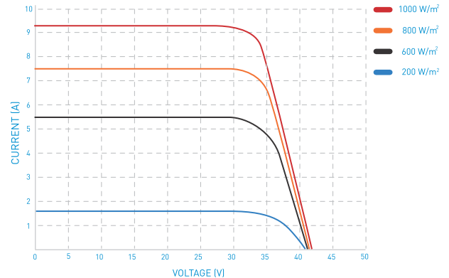
Typical IV Curves
